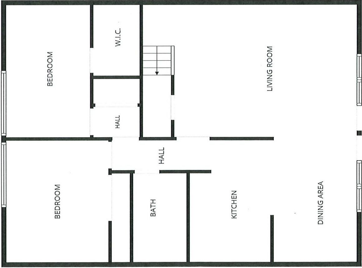
1st floor
