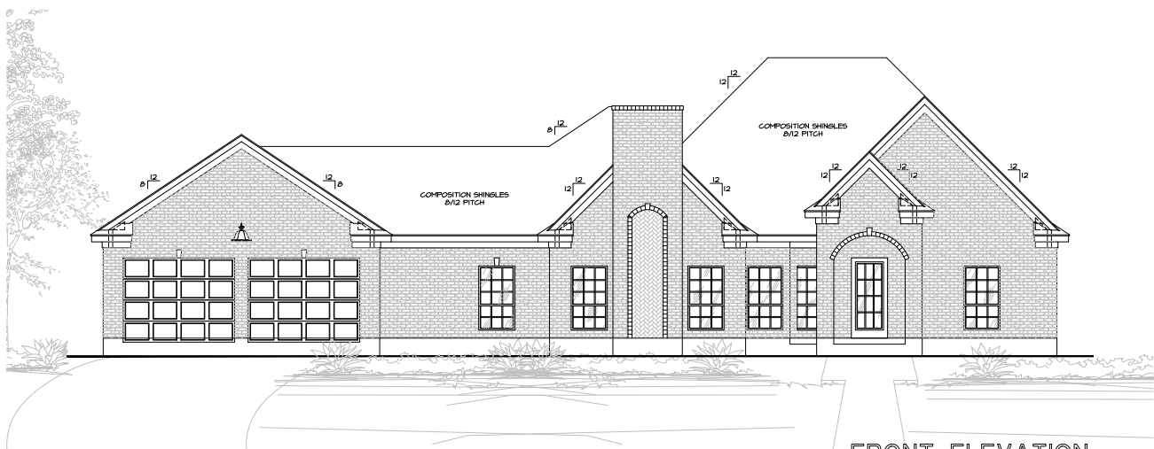
FRONT ELEVATION
