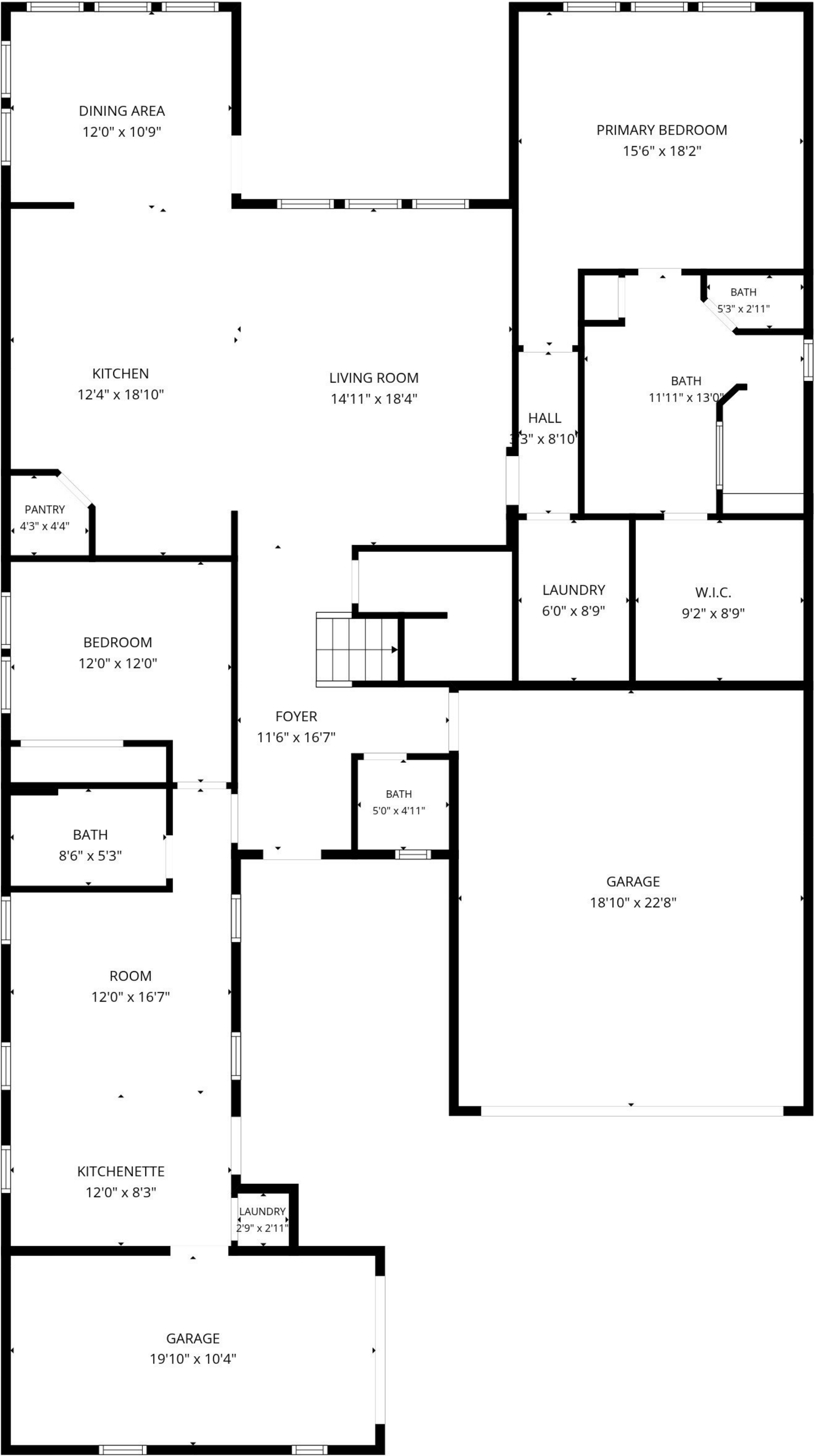
1st floor
