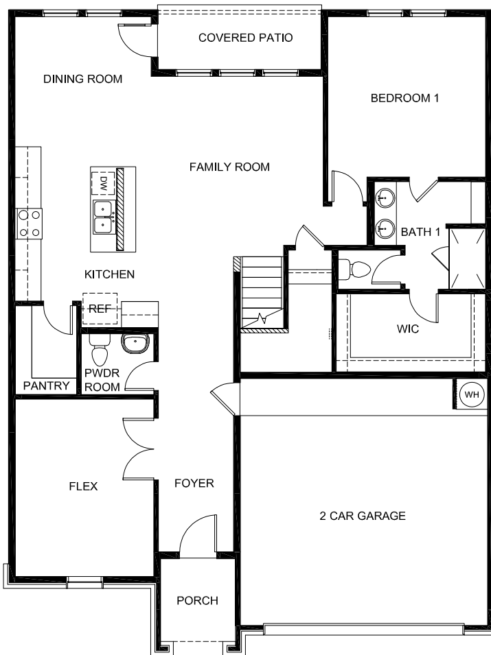
1ST FLOOR PLAN C
