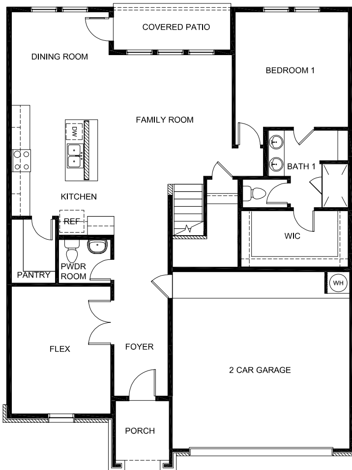
1ST FLOOR PLAN D
