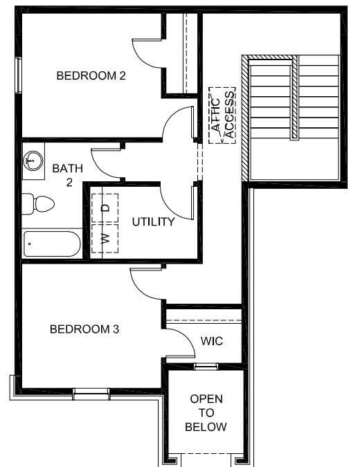
2ND FLOOR PLAN C
