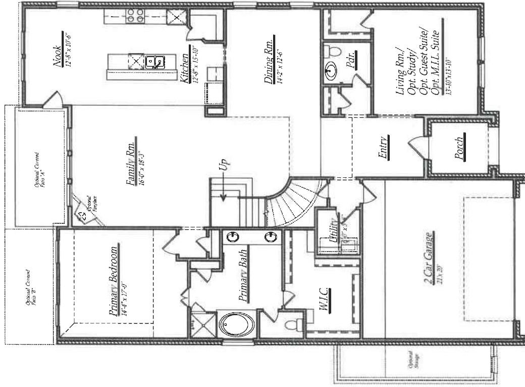
First Floor
