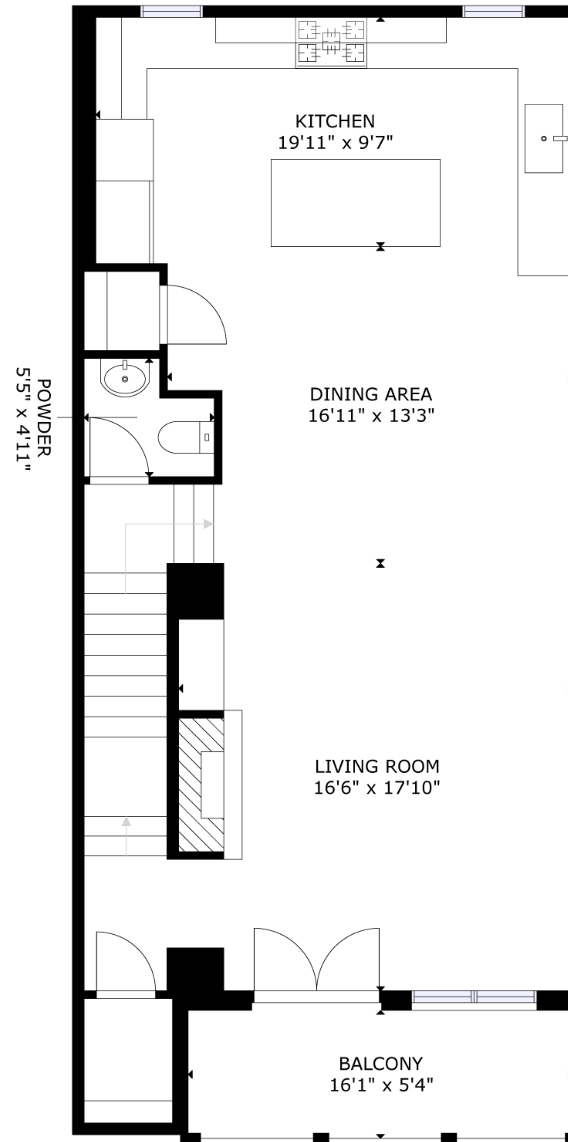
FLOOR 2
