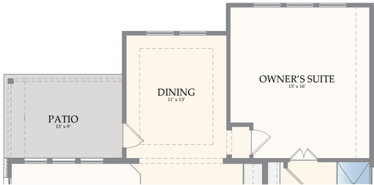
OPT. 3' EXTENSION @ OWNER'S SUITE
