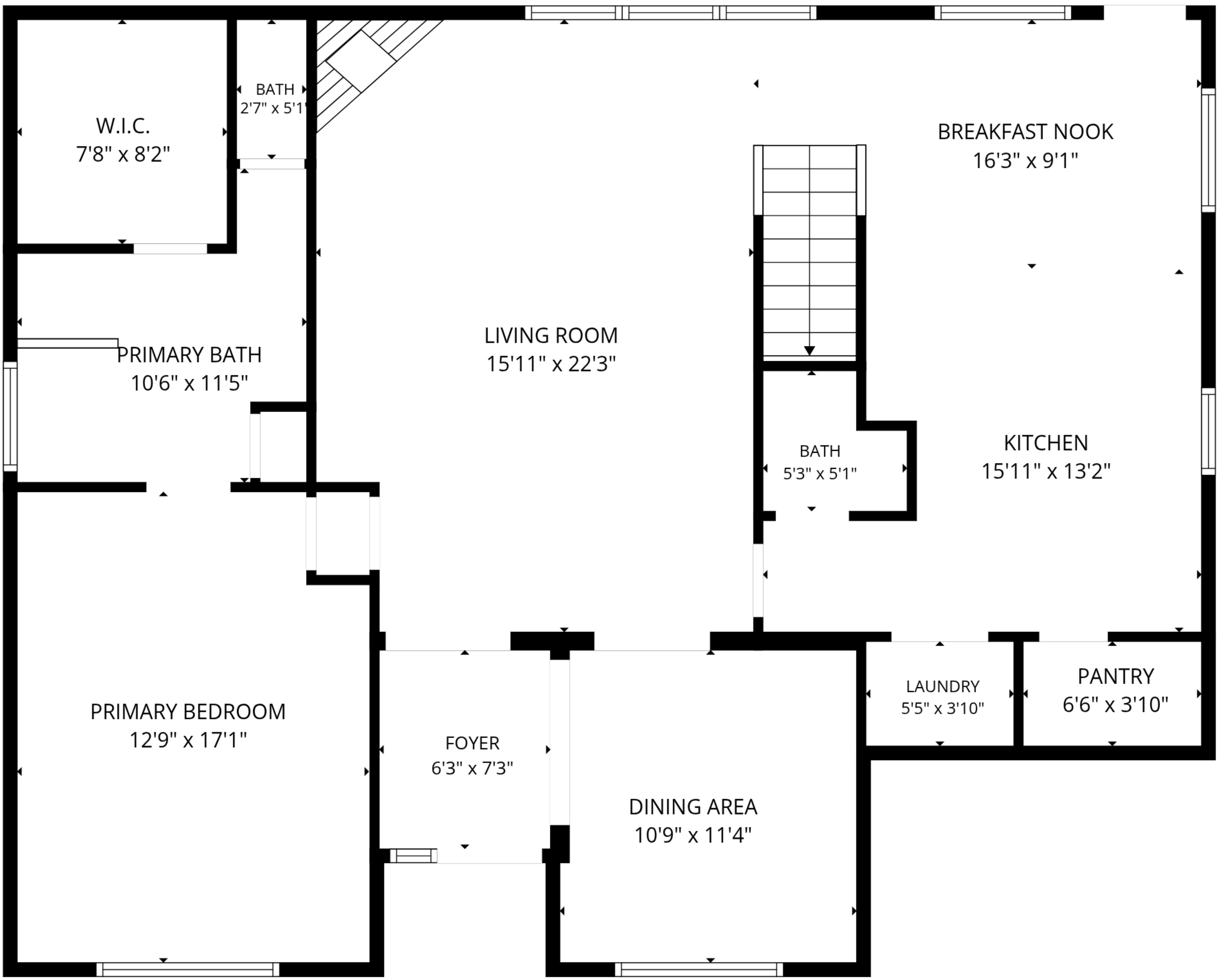
1st floor
