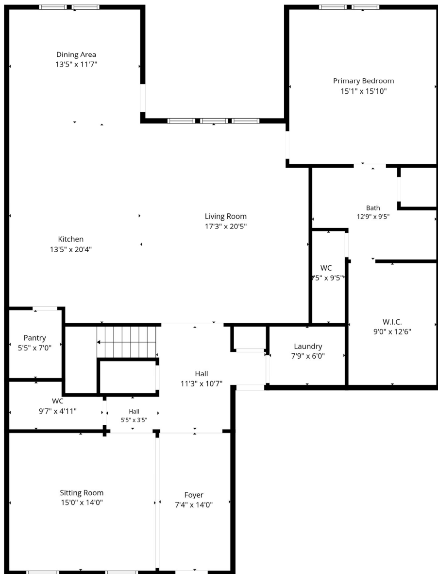
Ground Floor
