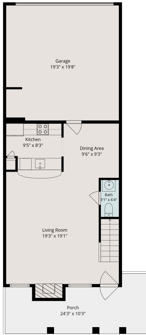
1st Floor
