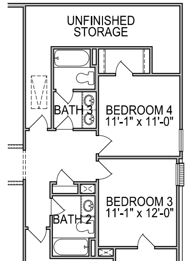
SECOND FLOOR PLAN OPT. #0486 ALT. BATH 2 LAYOUT
