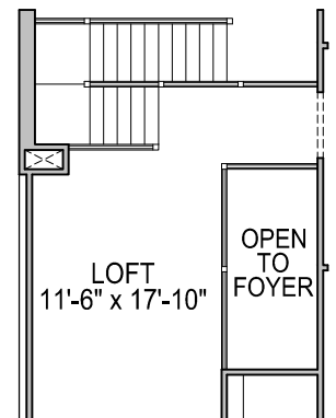
SECOND FLOOR PLAN OPT. #0050 RAILING
