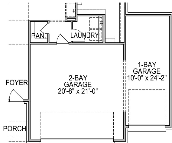
FIRST FLOOR PLAN OPT. #0593 1 BAY GARAGE
