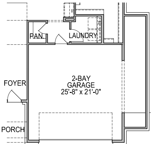
FIRST FLOOR PLAN OPT. #0613 5' GARAGE EXT.
