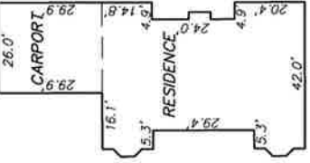
HOUSE DETAIL
