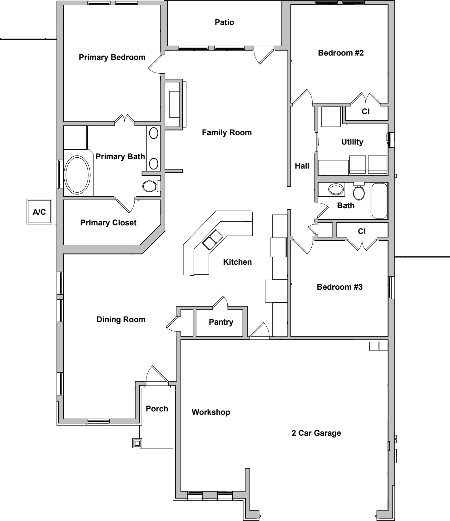
1 FLOOR PLAN 1/8" = 1'-0"
