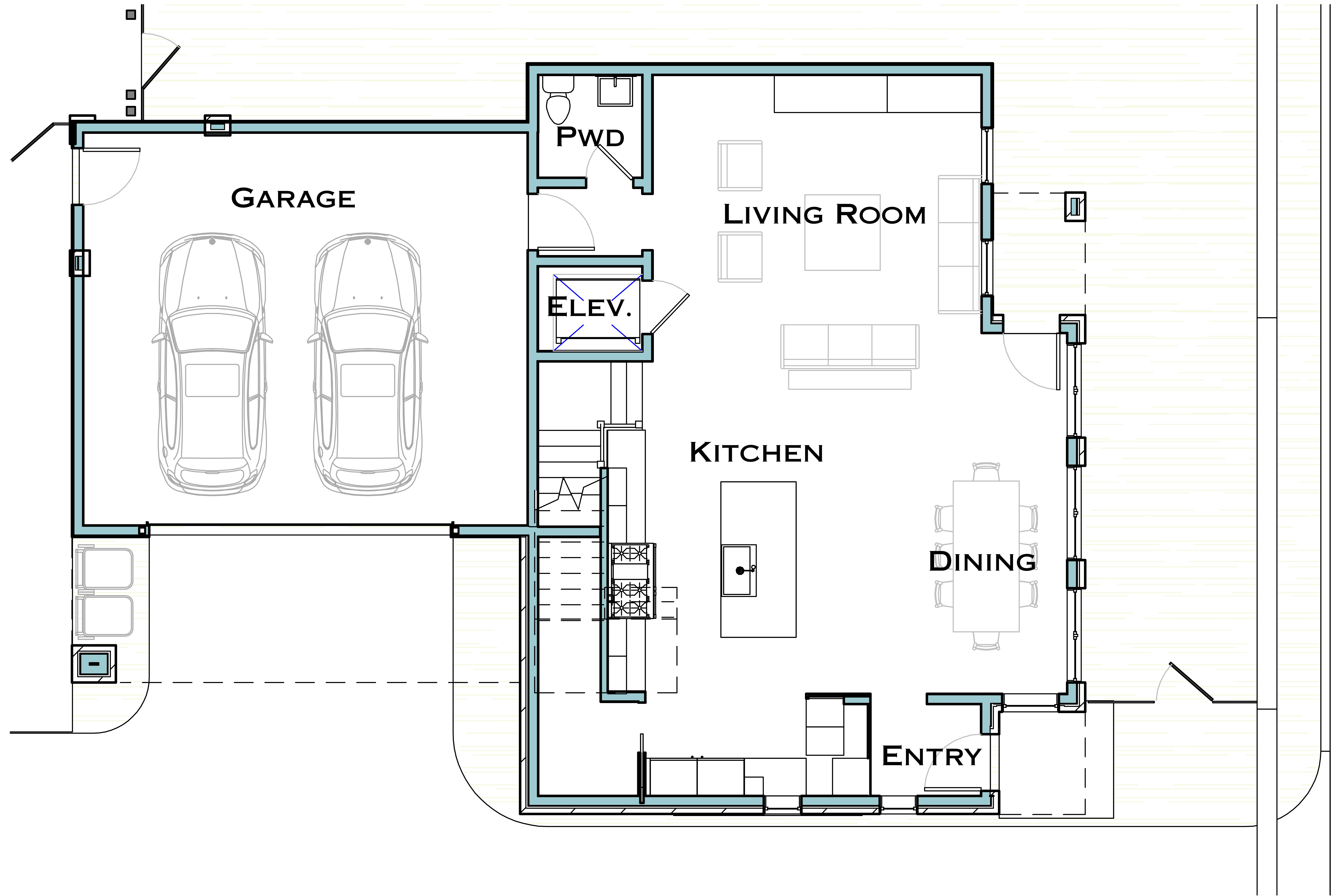
FIRST FLOOR
