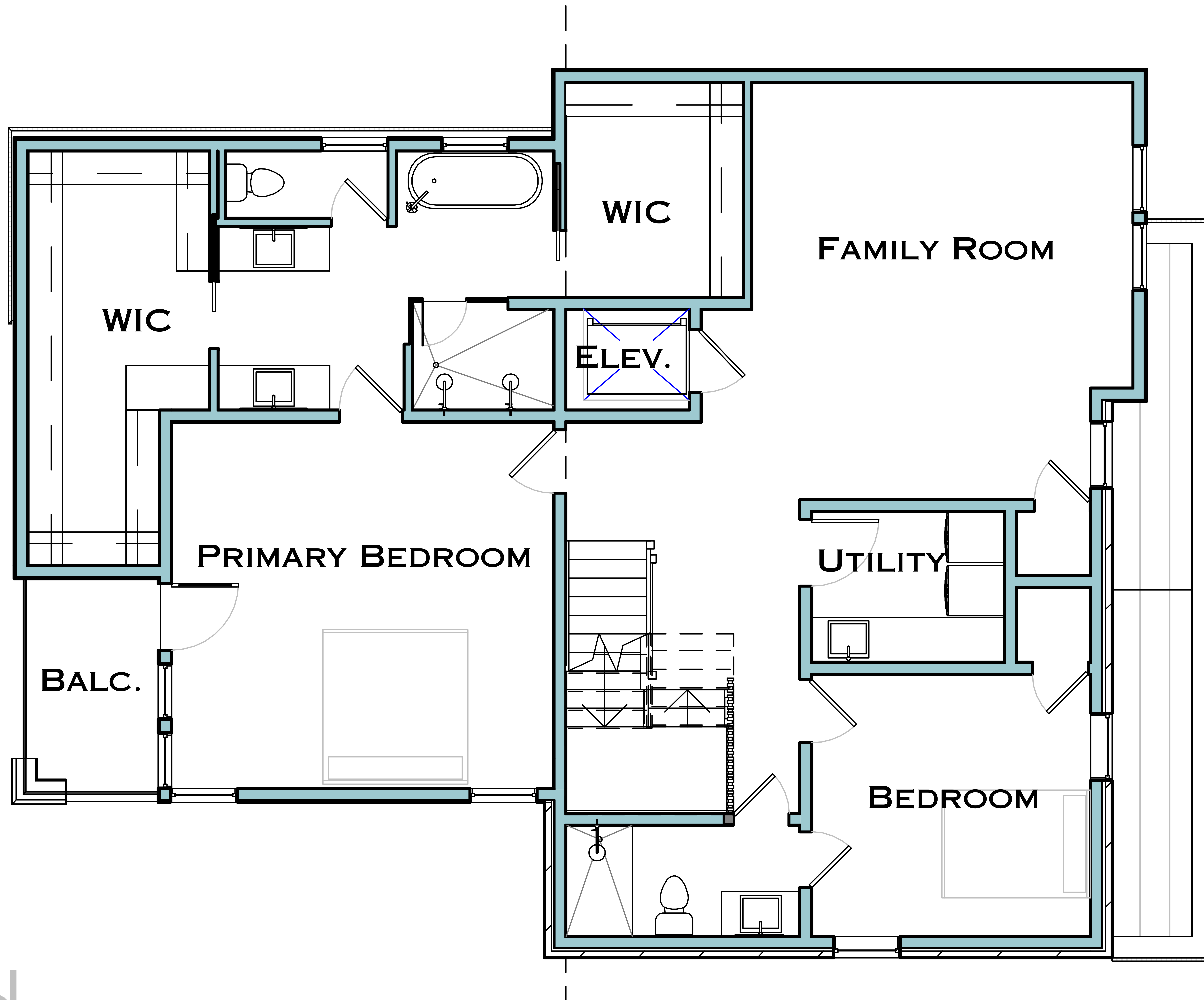
SECOND FLOOR
