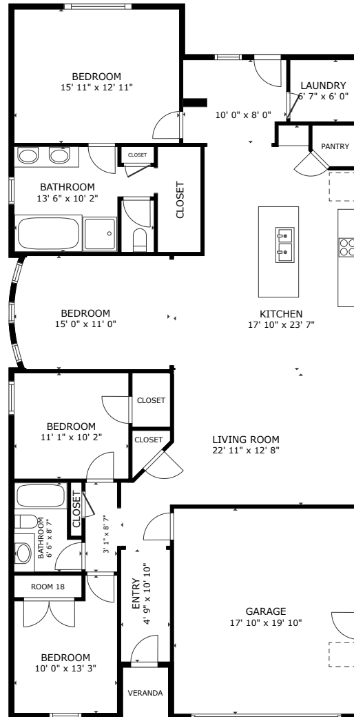
FLOOR PLAN
