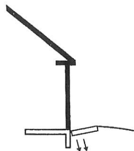
Flatwork Settlement
