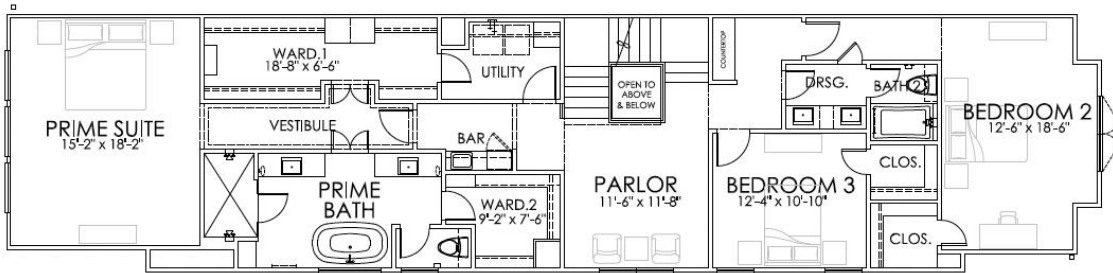
SECOND FLOOR
