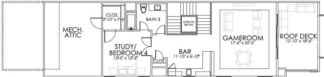
THIRD FLOOR
