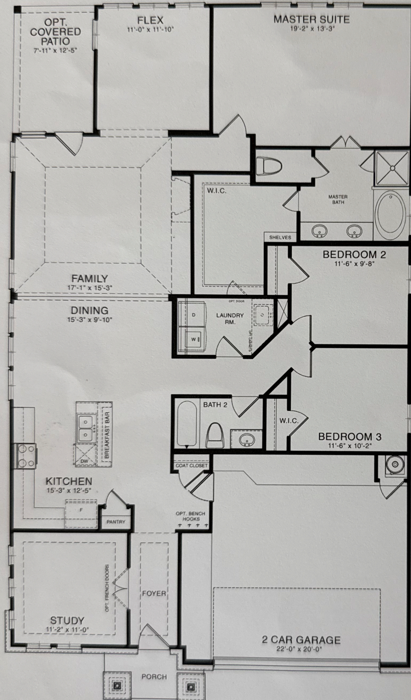
MAIN FLOOR PLAN ELEVATION A
