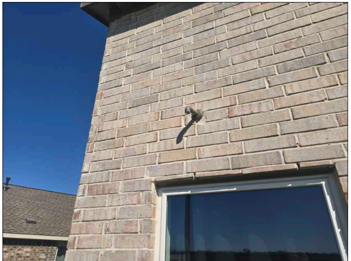
Secondary Drain line discharge location is over window. If water is seen coming from here, the primary may be stopped up. Contact HVAC service immediately to prevent possible damage.
