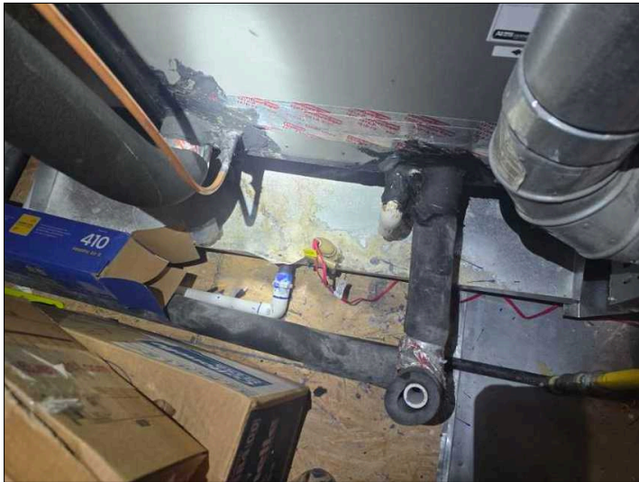
Trip switches present inside a/c condenser overflow pan. These detect water and will cause the unit to stop operating.
