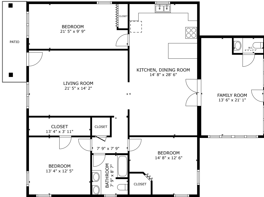
FLOOR PLAN
