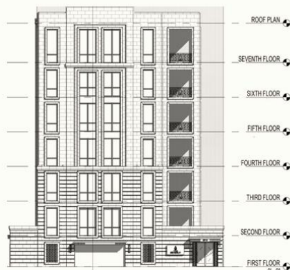
South Elevation
