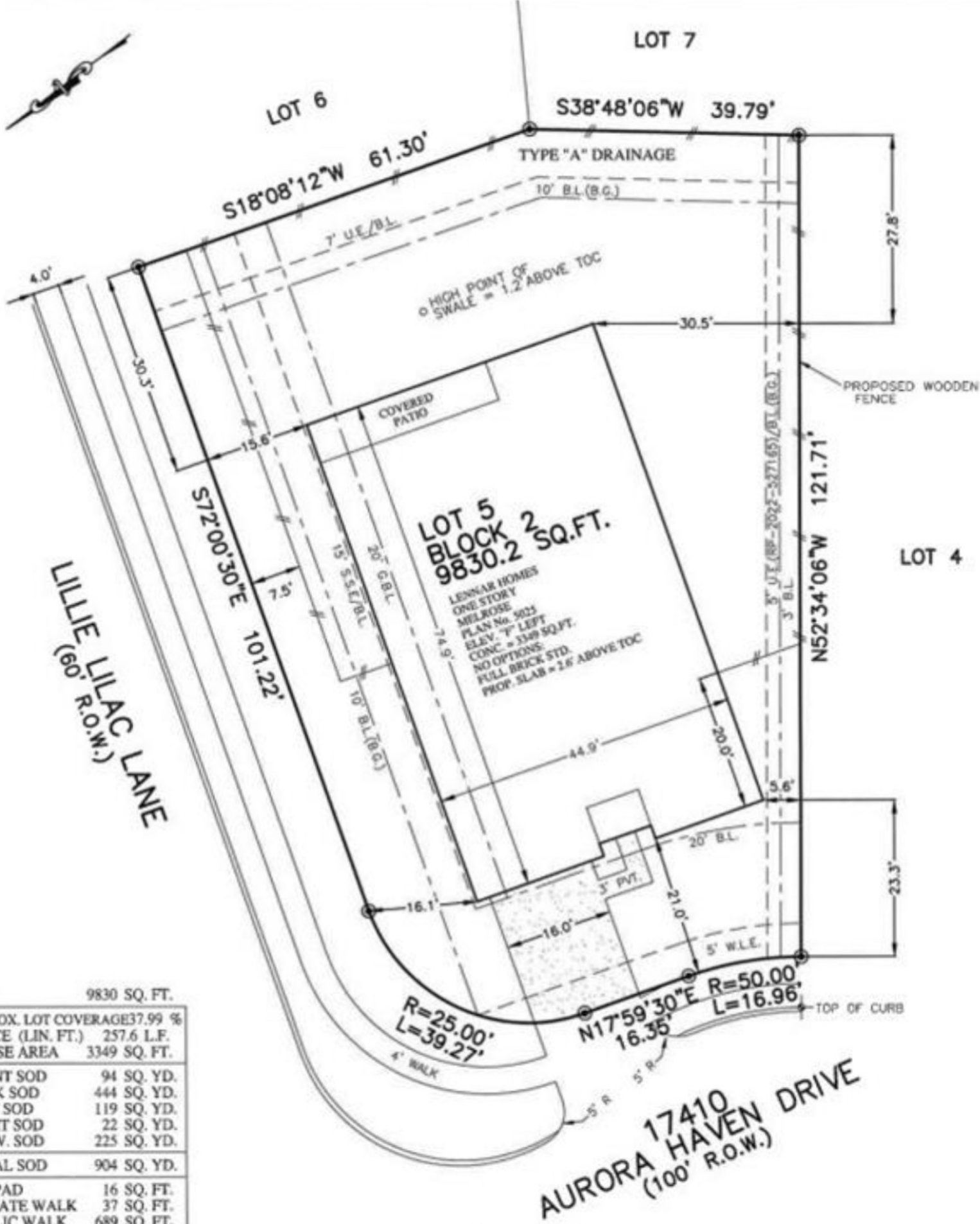
PLOT PLAN SCALE: 1" = 20'
