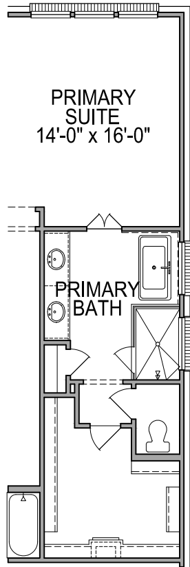
FIRST FLOOR PLAN OPT. #0073 5' FREE STANDING TUB
