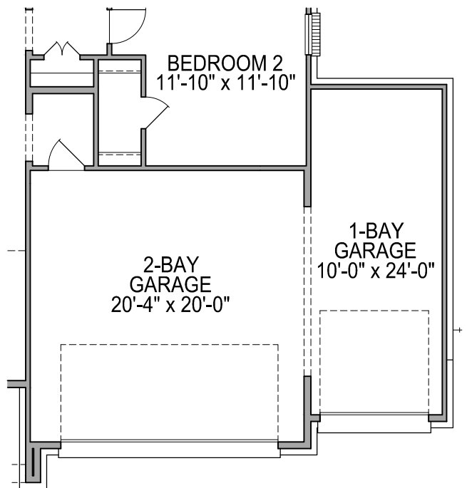
FIRST FLOOR PLAN OPT. #0593 1 BAY GARAGE
