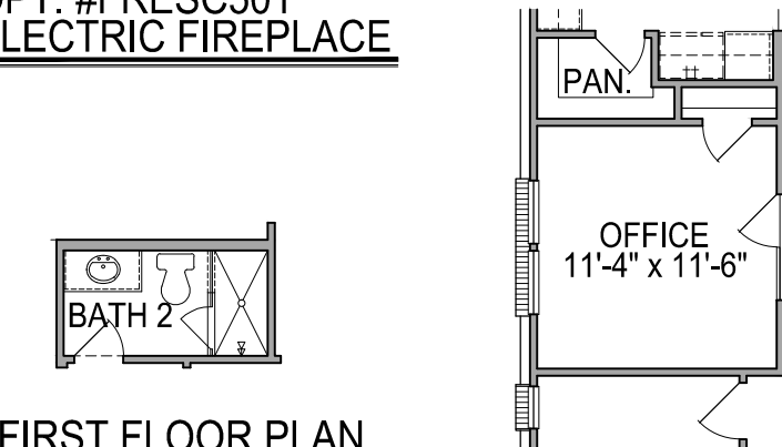
FIRST FLOOR PLAN OPT. #0569 OFFICE FROM FLEX
