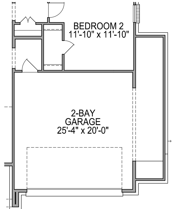
FIRST FLOOR PLAN OPT. #0613 5' GARAGE EXT.
