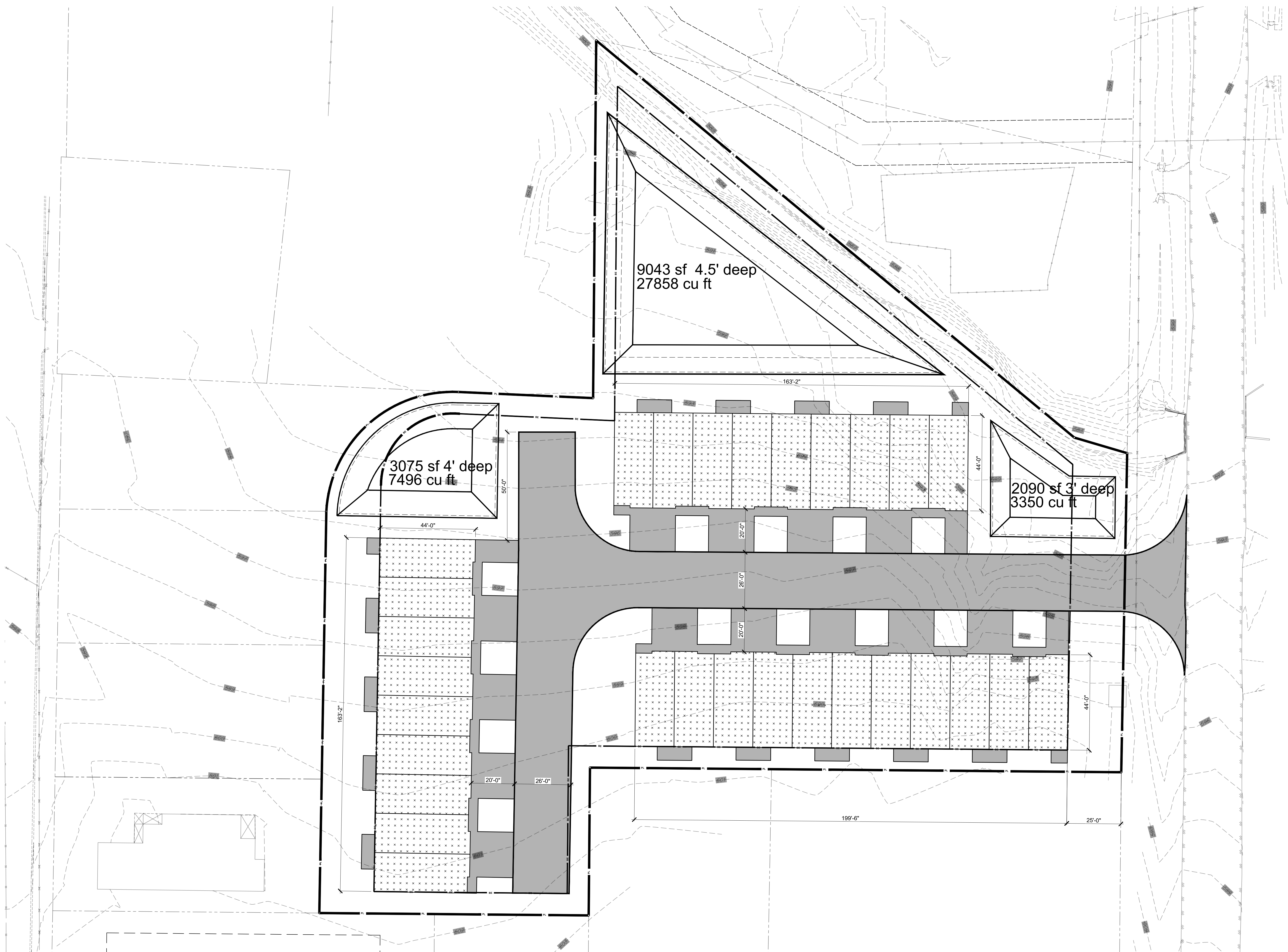
AP1 POD PLAN - FIRST FLOOR
