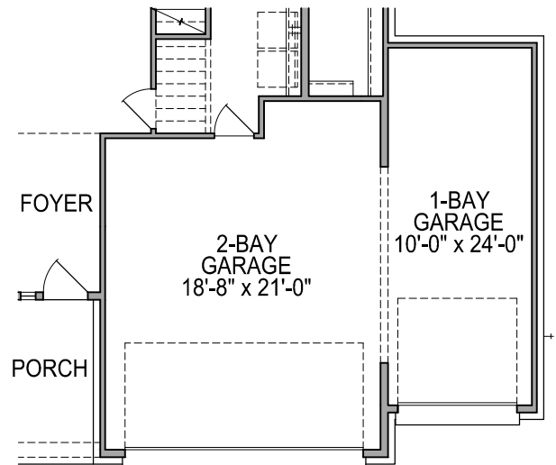
FIRST FLOOR PLAN OPT. #0593 1 BAY GARAGE
