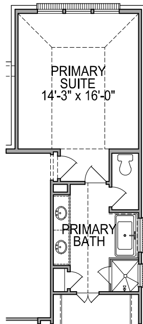
FIRST FLOOR PLAN OPT. #0073 5' FREE STANDING TUB
