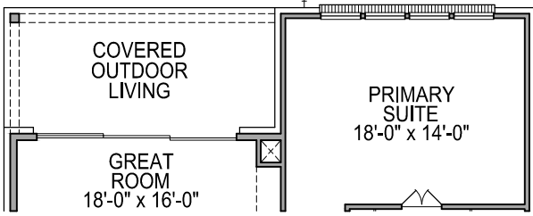
FIRST FLOOR PLAN OPT. #0790 SLIDERS @ GREAT ROOM
