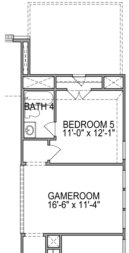
SECOND FLOOR PLAN OPT. #0094 BED 5/BATH 4 FROM ATTIC/GAMEROOM
