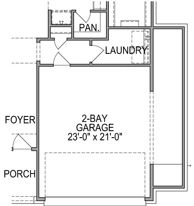
FIRST FLOOR PLAN OPT. #0613 5' GARAGE EXT.
