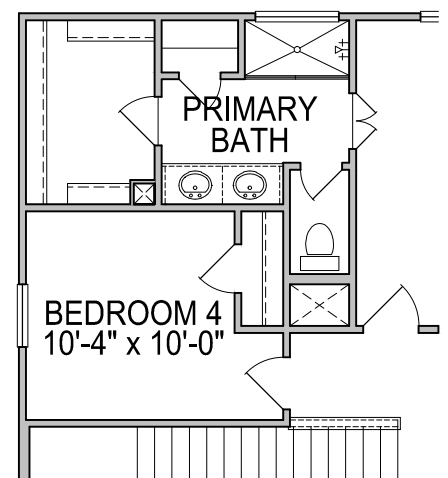
SECOND FLOOR PLAN OPT. #0322 BEDROOM 4 FROM LOFT
