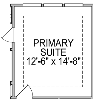
SECOND FLOOR PLAN OPT. #0668 PRIMARY SUITE COFFER
