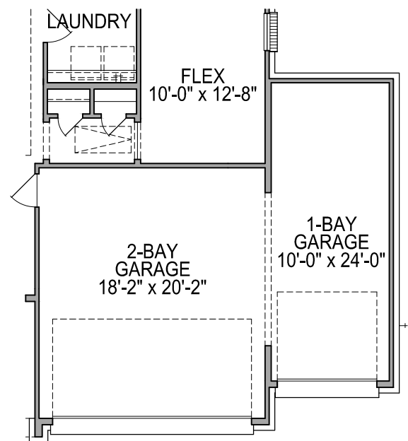
FIRST FLOOR PLAN OPT. #0593 1 BAY GARAGE
