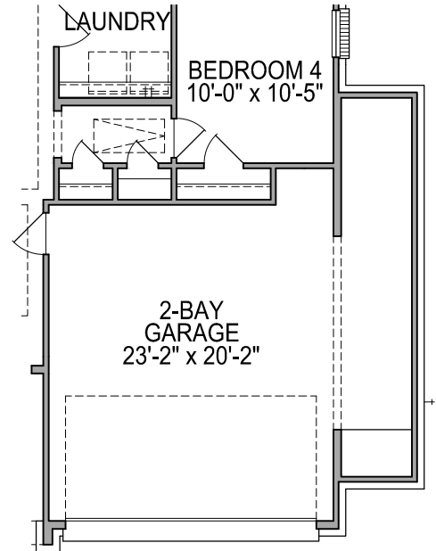
FIRST FLOOR PLAN OPT. #0733 BED 4/BATH 3 w/ #0613 5' GARAGE EXT. FROM FLEX
