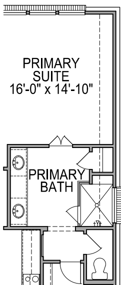
FIRST FLOOR PLAN OPT. #0072 LUXURY SHOWER
