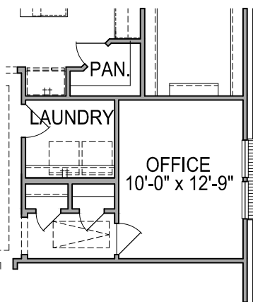
FIRST FLOOR PLAN OPT. #0569 OFFICE FROM FLEX
