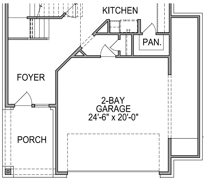
FIRST FLOOR PLAN OPT. #0613 5' GARAGE EXT.
