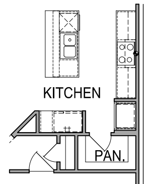
FIRST FLOOR PLAN OPT. #0161 36" COOKTOP W/ OVEN/MICRO TOWER CONFIGURATION
