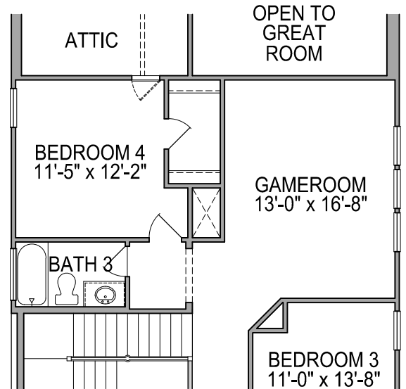
SECOND FLOOR PLAN OPT. #0400 BED 4/BATH 3 FROM ATTIC
