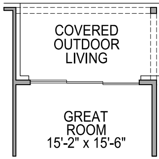
FIRST FLOOR PLAN OPT. #0795 COVERED OUTDOOR LIVING W/ GREAT ROOM SLIDERS
