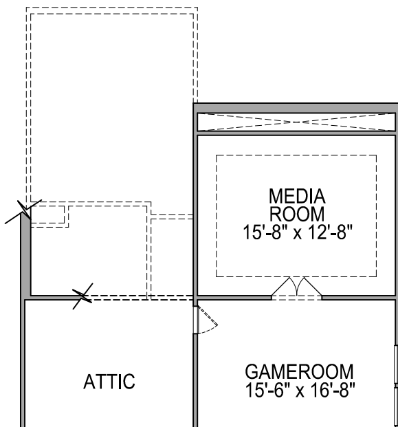
SECOND FLOOR PLAN OPT. #0526 MEDIA ROOM
