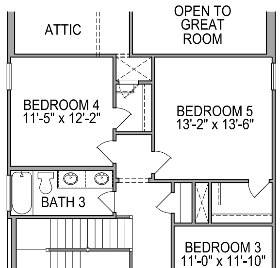
SECOND FLOOR PLAN OPT. #0459 BED 4 & 5/BATH 3
