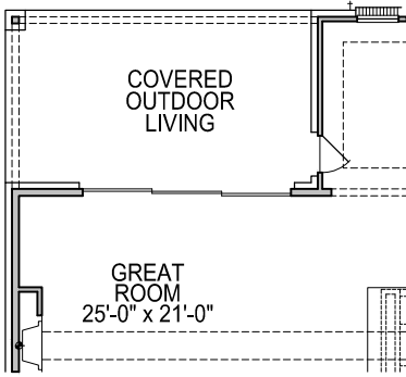
FIRST FLOOR PLAN OPT. #0790 SLIDERS @ GREAT ROOM
