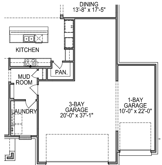
FIRST FLOOR PLAN OPT. #0593 1 BAY GARAGE
