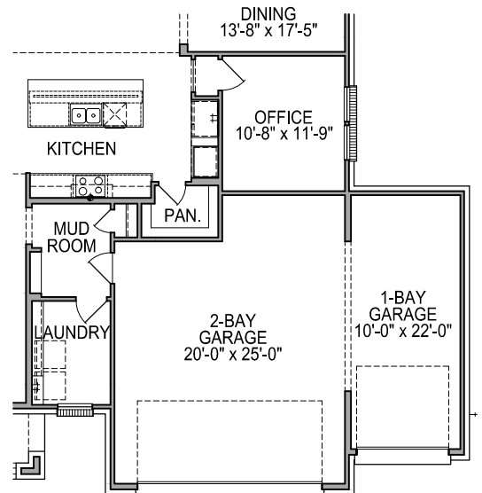
FIRST FLOOR PLAN OPT. #0593 1 BAY GARAGE w/ OPT. #0576 OFFICE OR OPT. #0485 PREP KITCHEN FROM GARAGE
