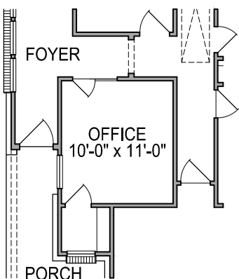
FIRST FLOOR PLAN OPT. #0569 OFFICE FROM FLEX
