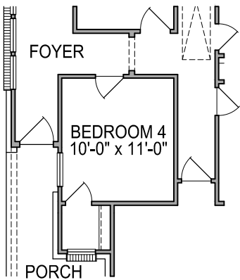
FIRST FLOOR PLAN OPT. #0426 BEDROOM 4 FROM FLEX
