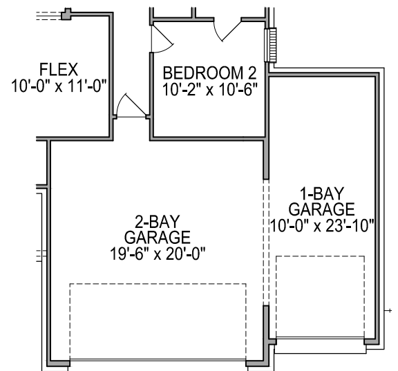
FIRST FLOOR PLAN OPT. #0593 1 BAY GARAGE
