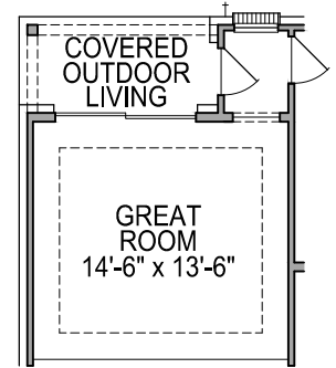
FIRST FLOOR PLAN OPT. #0790 SLIDERS @ GREAT ROOM
