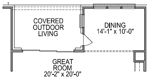
FIRST FLOOR PLAN OPT. #0790 GLASS SLIDERS @ GREAT ROOM
