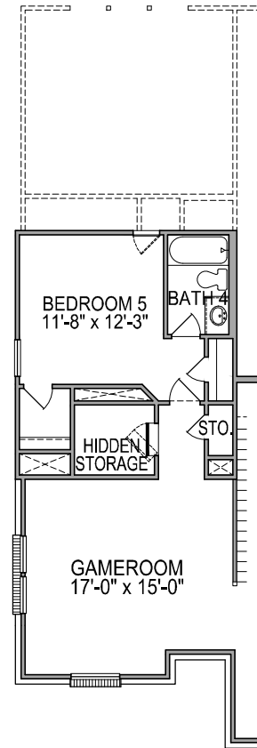
SECOND FLOOR PLAN OPT. #0094 BED 5/BATH 4 FROM ATTIC
