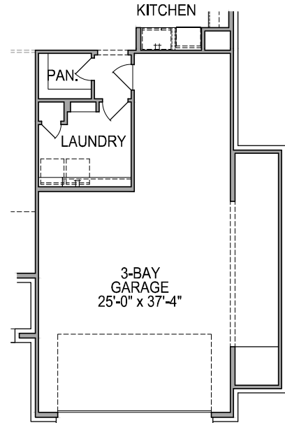
FIRST FLOOR PLAN OPT. #0613 5' GARAGE EXT.
