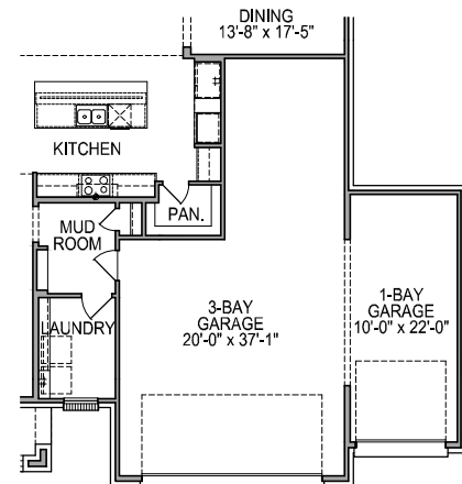
FIRST FLOOR PLAN OPT. #0593 1 BAY GARAGE
