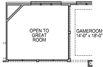
SECOND FLOOR PLAN OPT. #0050 RAILING @ GAMEROOM
