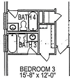
FIRST FLOOR PLAN OPT. #0340 BATH 4
