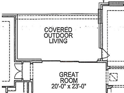
FIRST FLOOR PLAN OPT. #0790 SLIDERS @ GREAT ROOM
