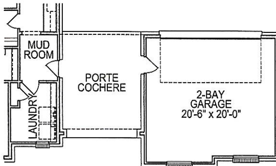
FIRST FLOOR PLAN OPT. #0215 2-BAY GARAGE
