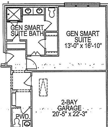
FIRST FLOOR PLAN OPT. #0794 SLIDERS @ GAMEROOM
