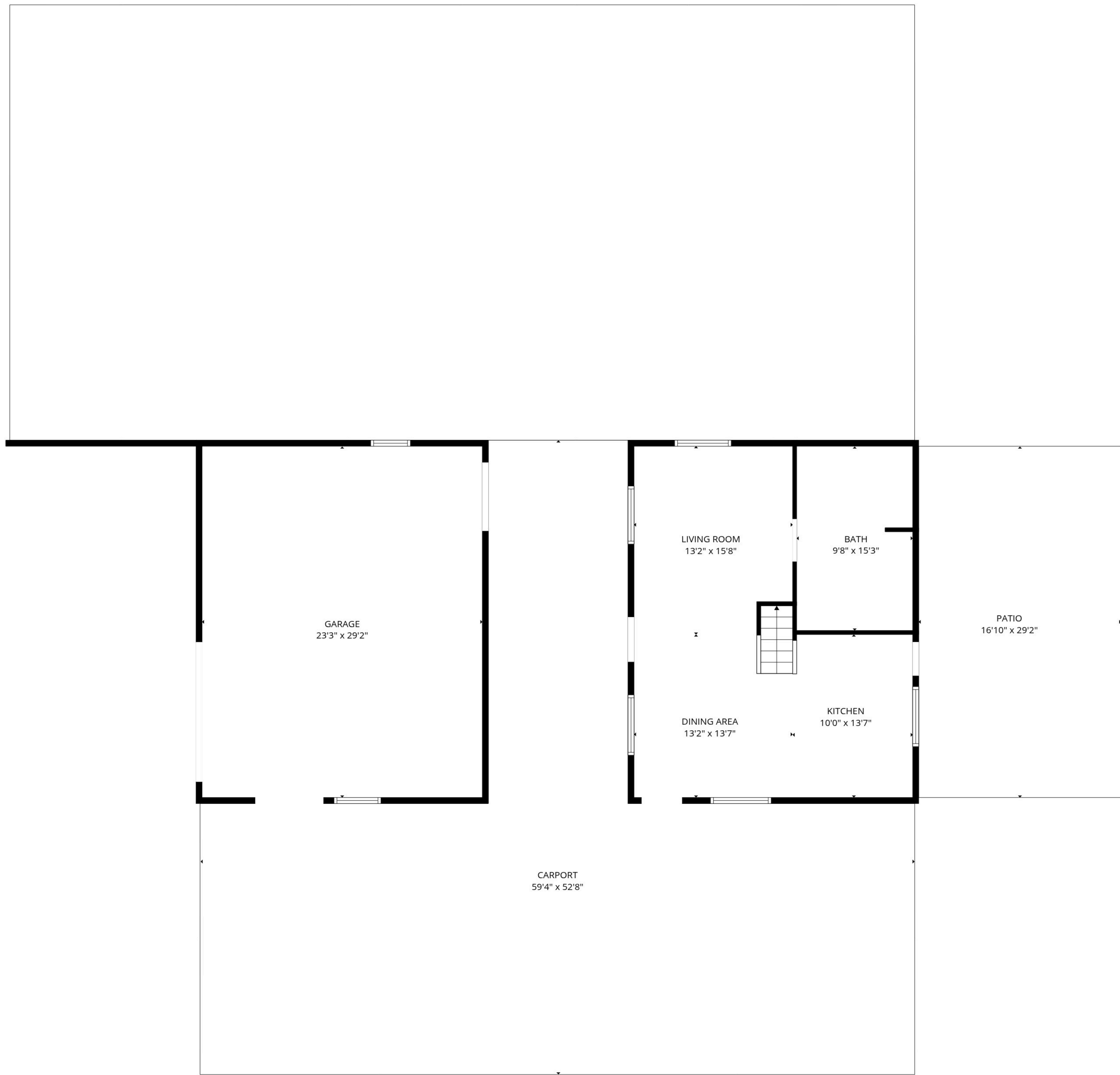
1st floor
