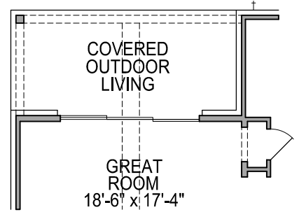
FIRST FLOOR PLAN OPT. #0790 SLIDERS @ GREAT ROOM
