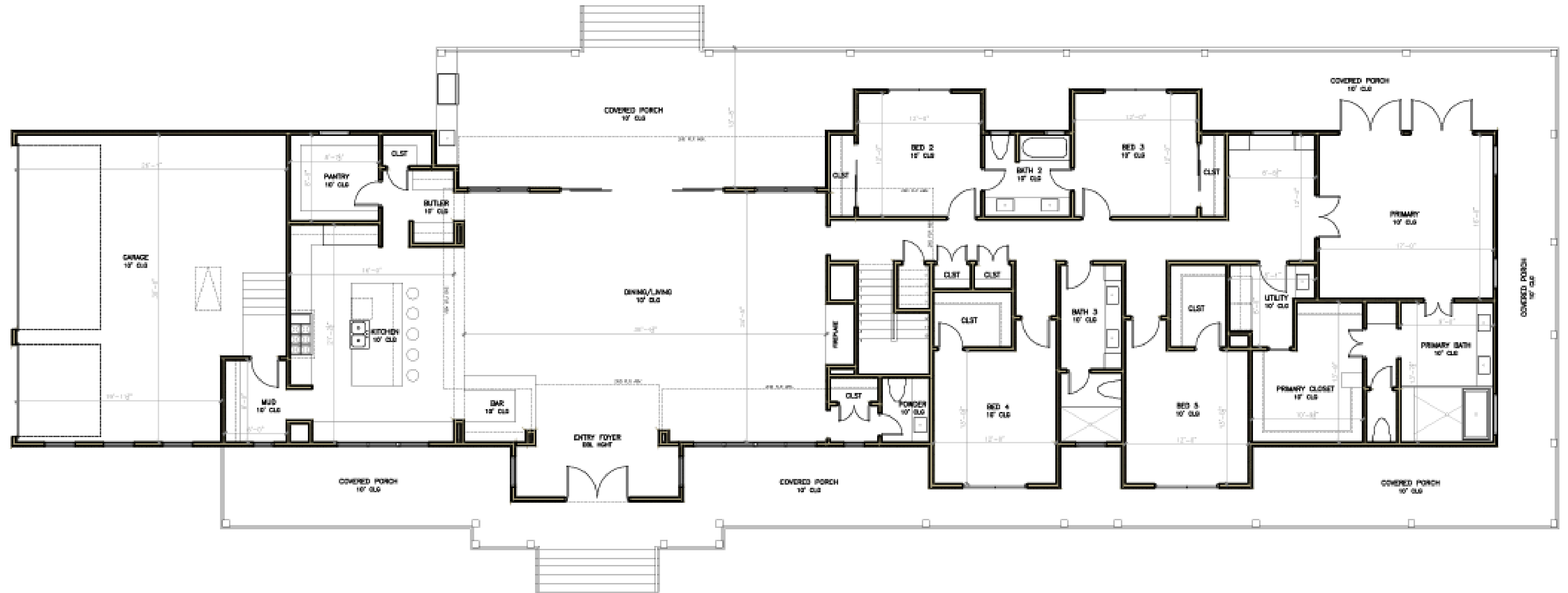
FIRST FLOOR SCALE: 3/32" = 1'-0"
