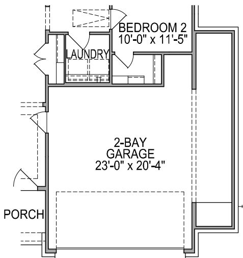
FIRST FLOOR PLAN OPT. #0613 5' GARAGE EXT.
