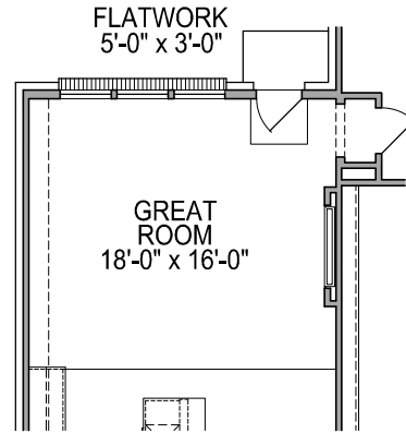
FIRST FLOOR PLAN OPT. #FRESC501 ELECTRIC FIREPLACE
