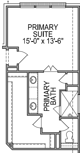
FIRST FLOOR PLAN OPT. #0072 LUXURY SHOWER
