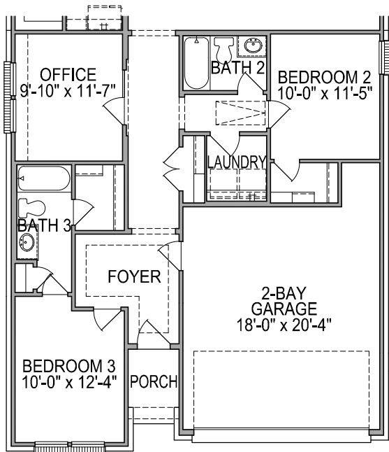
FIRST FLOOR PLAN OPT. #0653 OFFICE FROM BED 4
