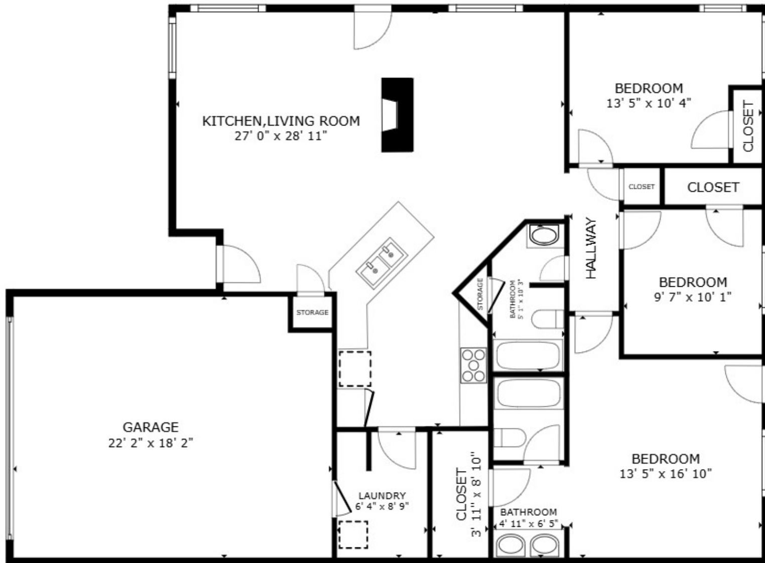
FLOOR PLAN
