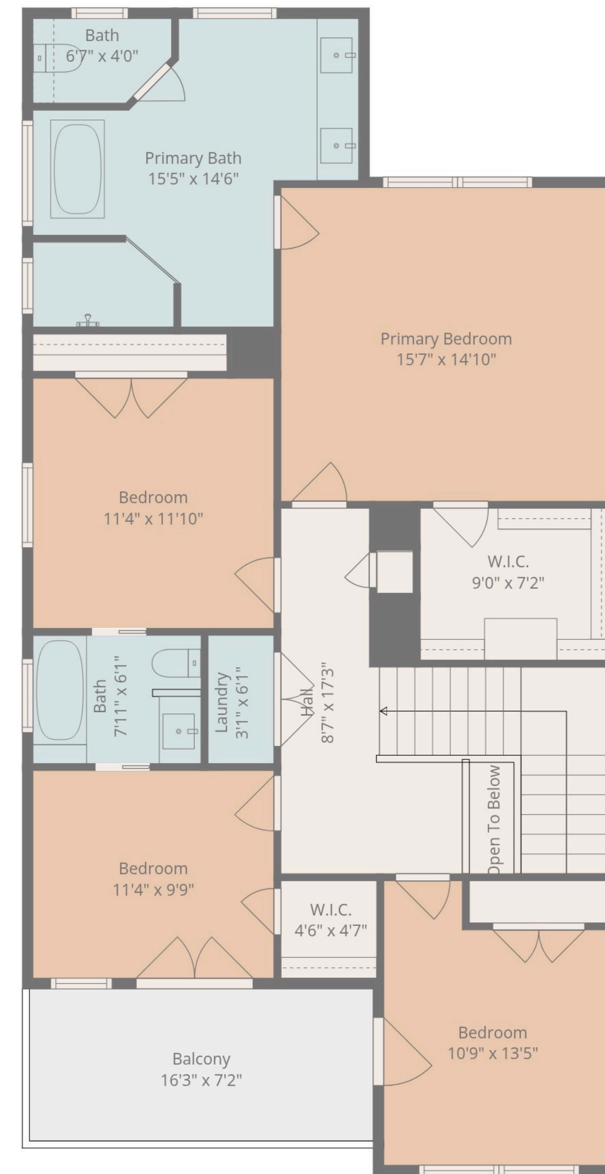
2nd Floor
