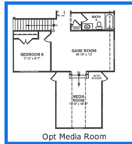
Opt Second Floor Plan
