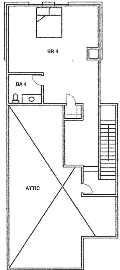
SECOND FLOOR
