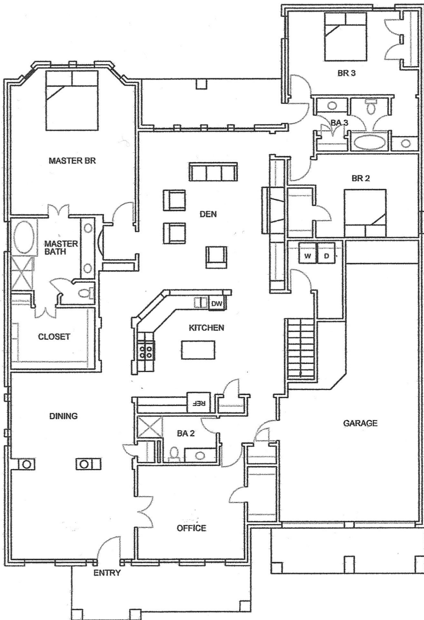
31 W CANYON WREN CIR FIRST FLOOR
