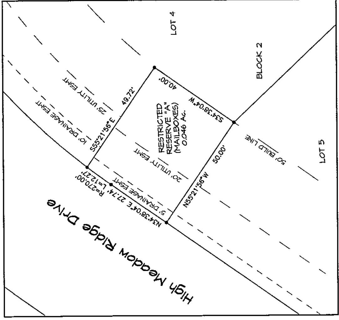
RESTRICTED RESERVE "A" DETAIL (MAILBOXES)
