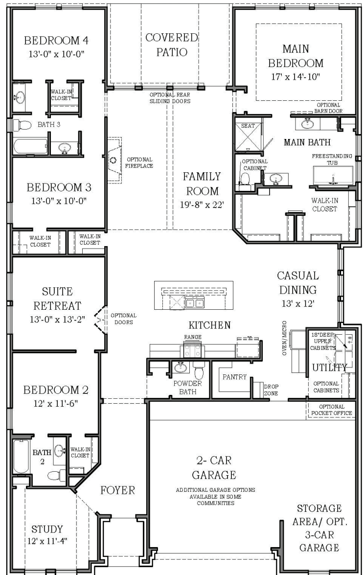
FLOOR PLAN
