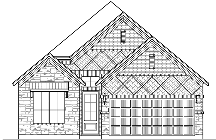
FRONT ELEVATION 'A1' STONE OPTION
