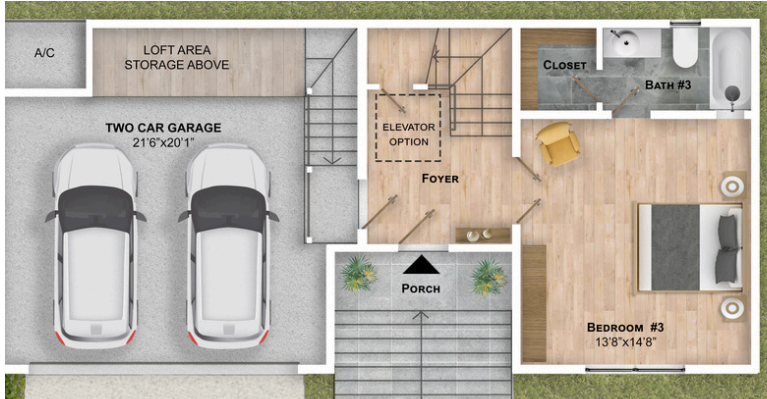
Level 1
