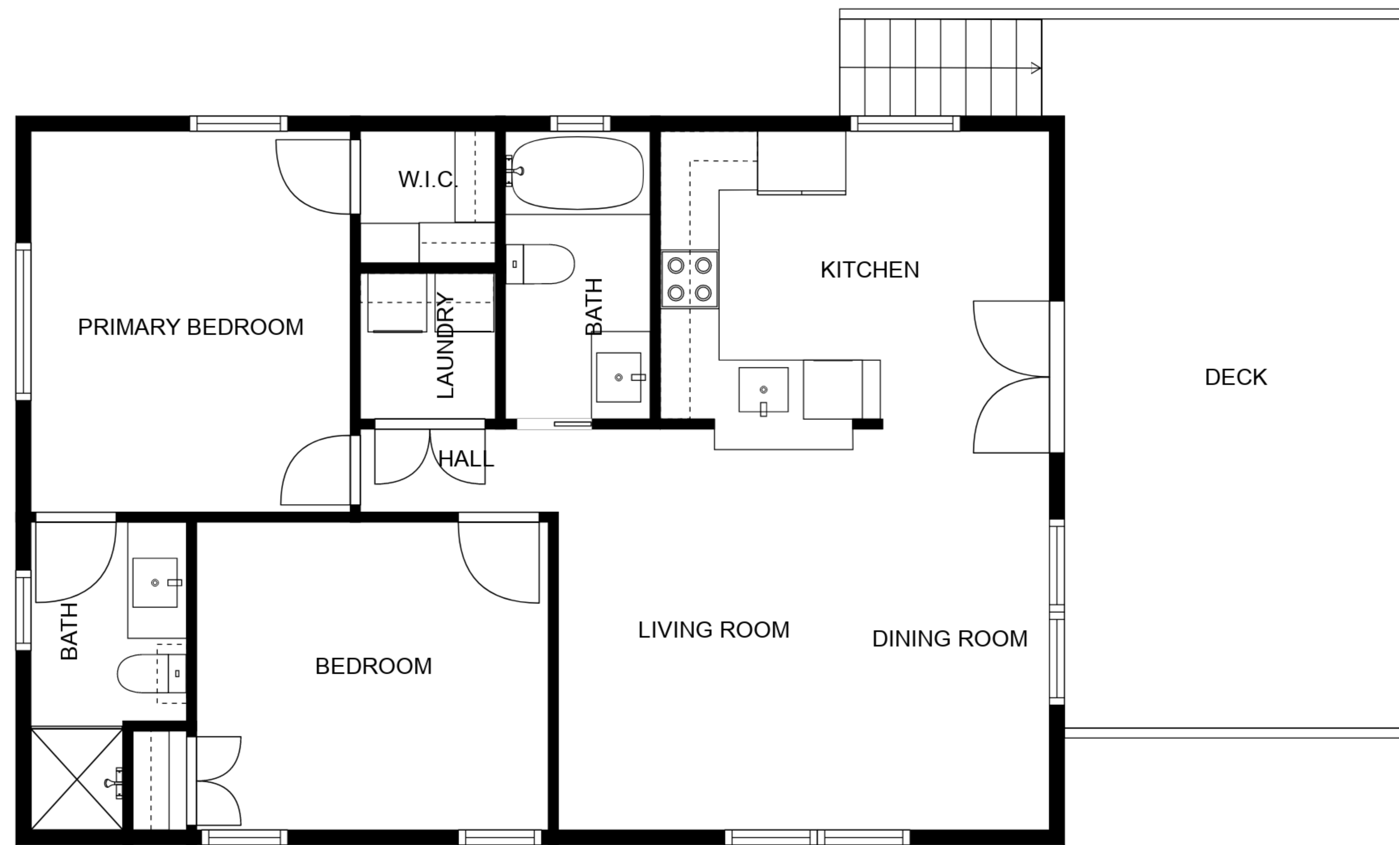
FLOOR 2
