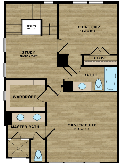
THIRD FLOOR
